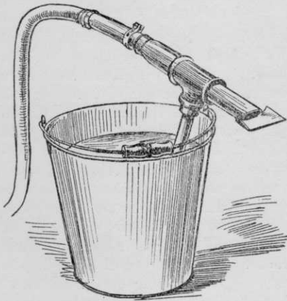
HYDRAULIC APPLICATOR, As Devised by Mr. Sturtevant.
